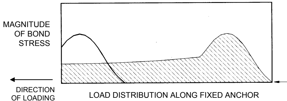
Figure 3. Load distribution and progressive debonding in conventional anchors.
