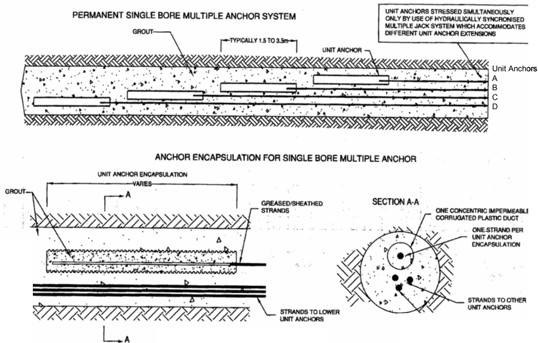
Figure 2. Elevations and cross section of a typical 4-unit SBMA.
