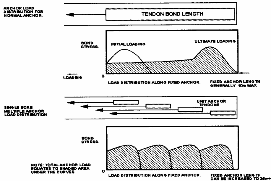
Figure 4. Comparison of load distribution along a conventional anchor and an SBMA (Barley, 2000).
