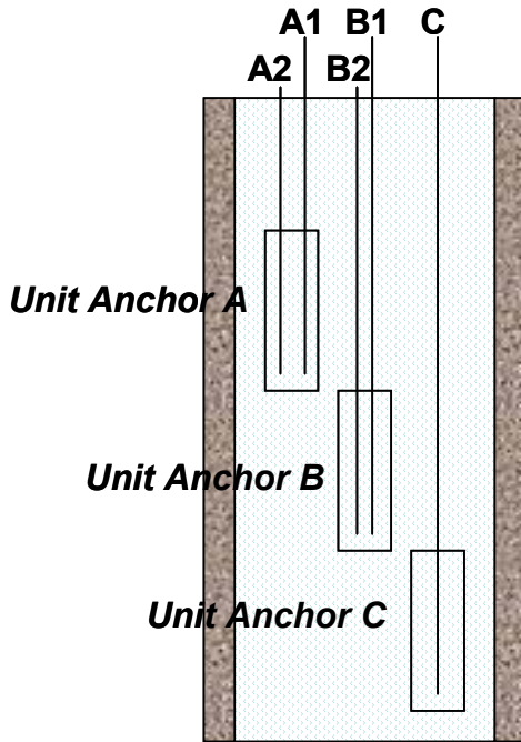
Figure 6. Stressing sequence for sacrificial anchor.
