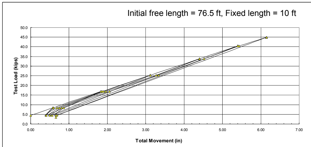
Figure 7. Total movement vs. load for Unit Anchor C during the Performance and Extended Creep Test.
