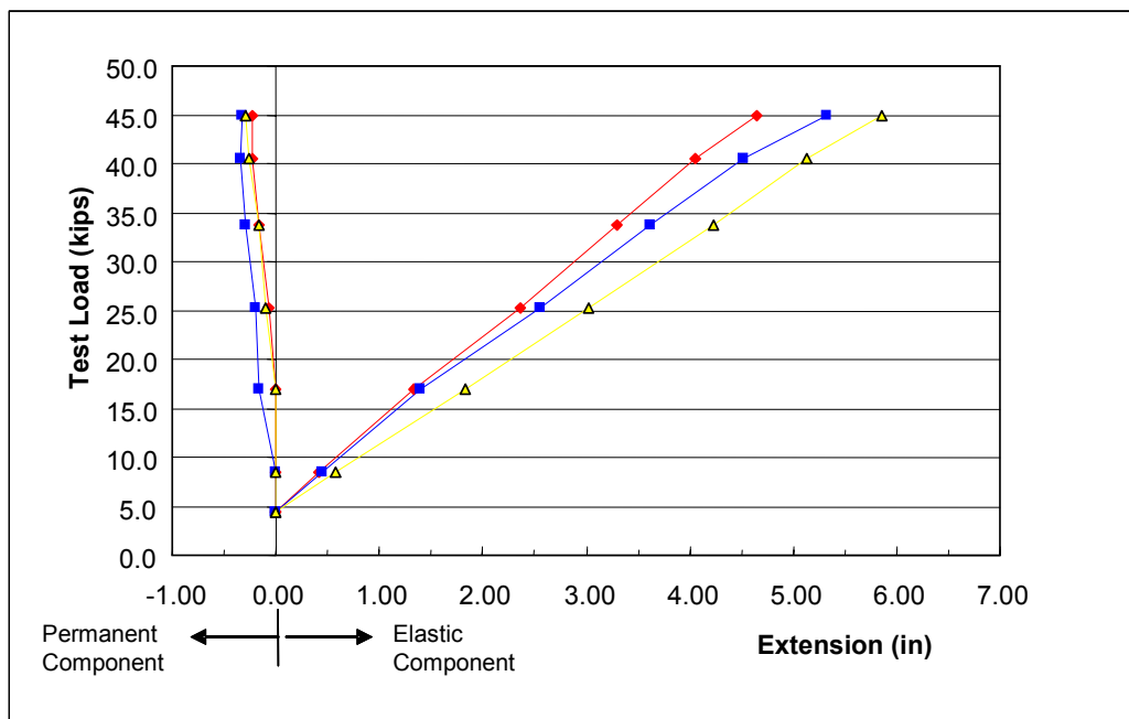
◆ Strand A1 (Initial free stressing length = 60.5 feet); ■ Strand B1 (Initial free stressing length = 70.5 feet); △ Strand C (Initial free stressing length = 80.5 feet)
